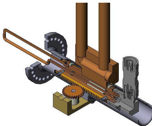
Figure 5: A cut-away rendering of the Mark IV coupling loop.
