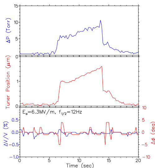
Figure 3: Tuner response to forced helium pressure fluctuation ( \frac{\Delta f}{\Delta P} = 1\text{Hz/Torr} ) and corresponding voltage (blue) and phase (red) errors for high field ( E_a=6.3 MV/m) and a bandwidth of \pm 12 Hz.
