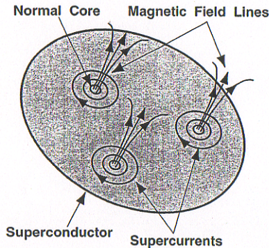
Figure 1: Flux trapping at imperfection in a superconducting material (copied from the ref.[1]).
