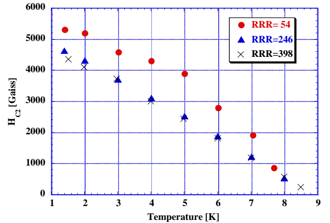
Figure 2: RRR dependence of H_{c2} on niobium.
